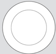
FLAT PLATE A 02/0101 Ø 27.5 cm. (10 7/8 ) 560 g. A 02/0102 Ø 21.5 cm. (8 1/2 ) 270 g. A 02/0103 Ø 17.5 cm. (6 7/8 ) 172 g.
